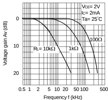
Fig.11 Frequency Response
